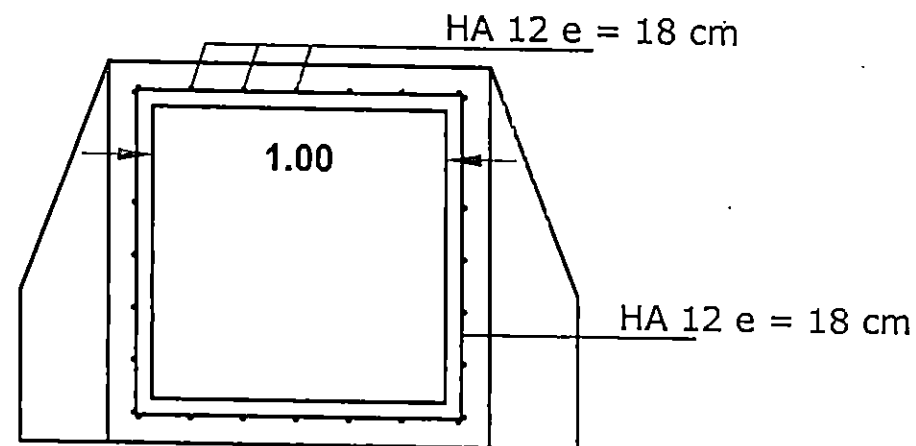
REINFORCEMENT SECTION A-A
